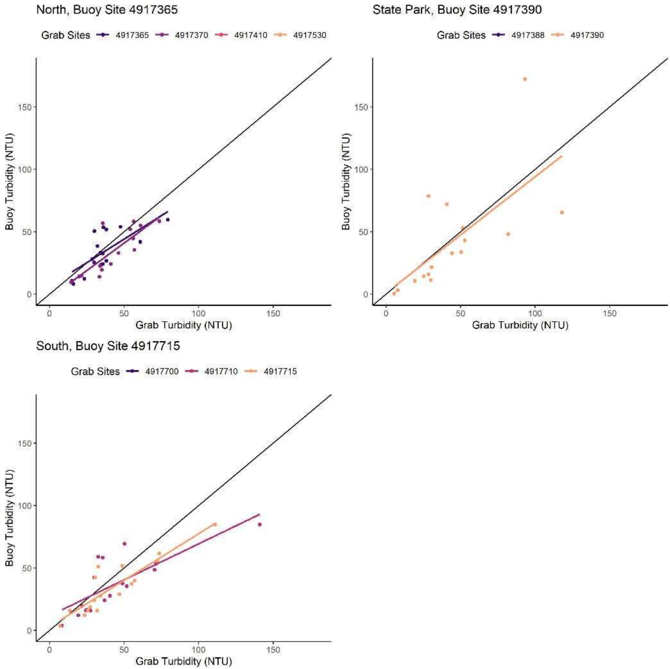
Figure 2.3.6. Comparisons of turbidity measured at buoy and grab sampling sites. Turbidity was not measured at the Provo Bay site (4917446). Grab sites correspond to sites near the buoy site, which did not necessarily have data available. A direct match in site code indicates grab and buoy samples were taken at the same location. NTU = nephelometric turbidity units. The solid black line represents a 1:1 relationship.
