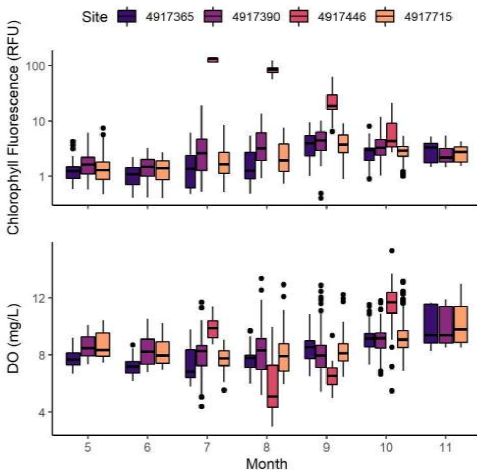
Figure 2.3.3. Monthly distributions of chlorophyll fluorescence and dissolved oxygen (DO) concentrations at buoy sites. Site codes are as follows: North = 4917365, State Park = 4917390, Provo Bay = 4917446, South = 4917715. RFU = relative fluorescence units, DO = dissolved oxygen.
