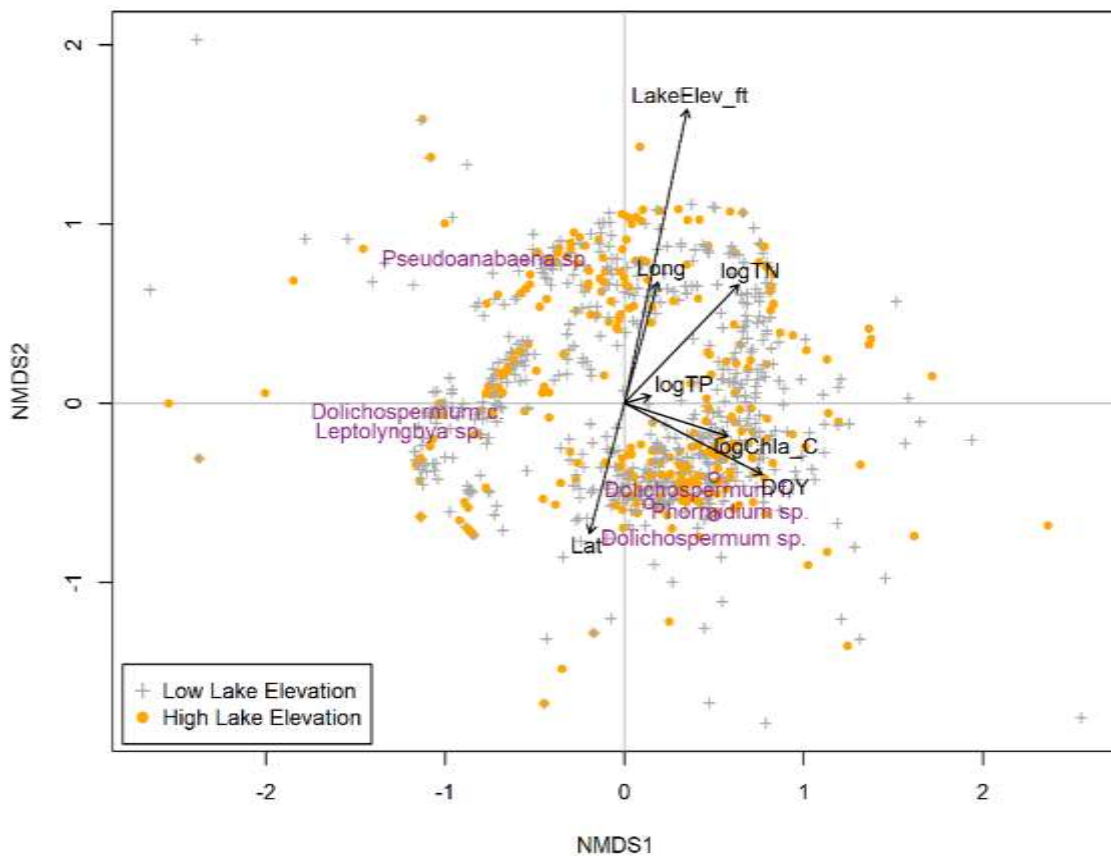
Figure 2.4.11. Non-metric multidimensional scaling (NMDS) relationships of individual samples (points; noted as either high or low lake elevation) and phytoplankton taxa (purple labels) as they relate to environmental variables (black vectors and labels). DOY = day of year, Long = longitude, Lat = latitude.
