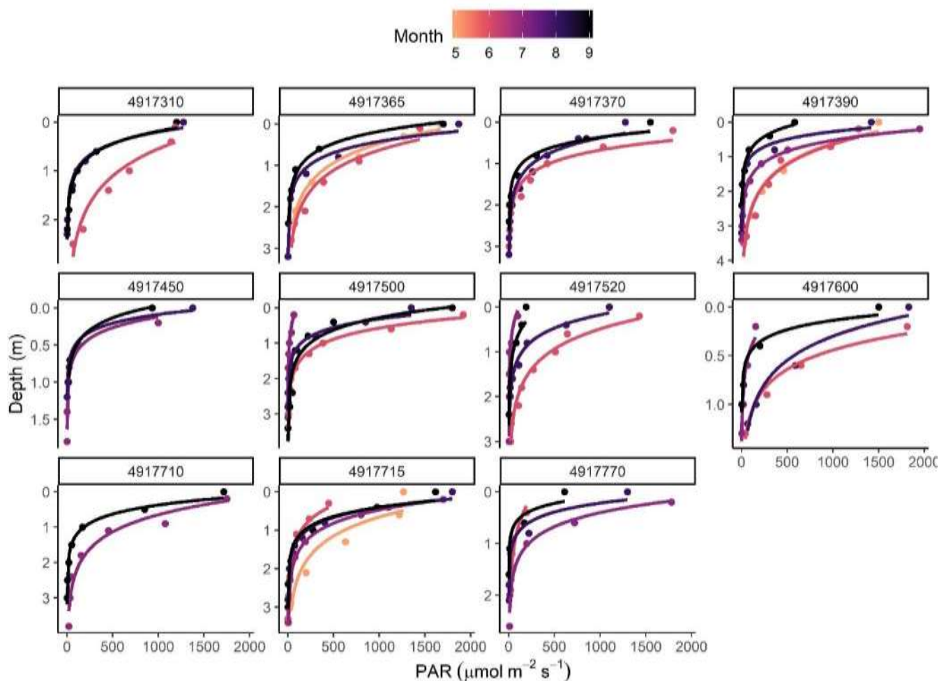
Figure 2.8.1. Attenuation of photosynthetically active radiation (PAR) with depth in Utah Lake. Panels represent sampling sites, with named sites as follows: North = 4917365, State Park = 4917390, South = 4917715.
