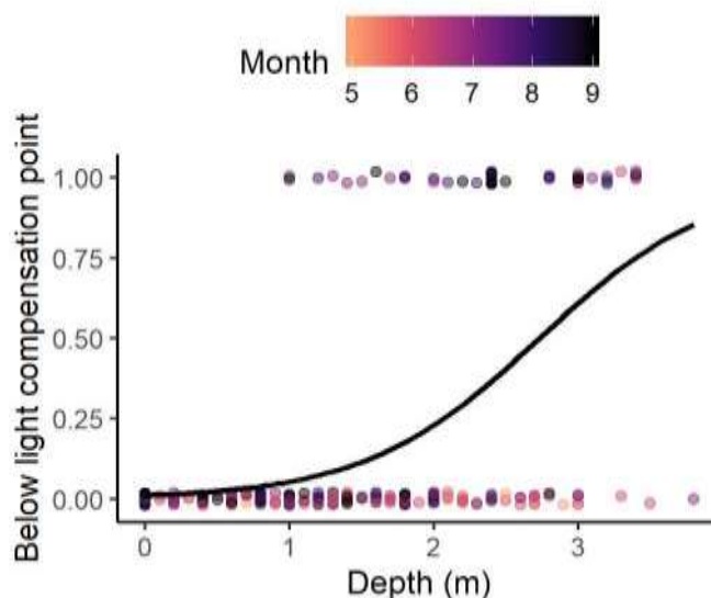
Figure 2.8.2. Logistic regression of water depth and samples above and below the light compensation point (0 and 1, respectively). The light compensation point was set at 10 \mu\text{mol m}^{-2} \text{s}^{-1} . The solid line represents the probability of a sample being below the light compensation point. Note: y axis values are either 0 or 1, but points are jittered to enable visualization of overlapping points.
