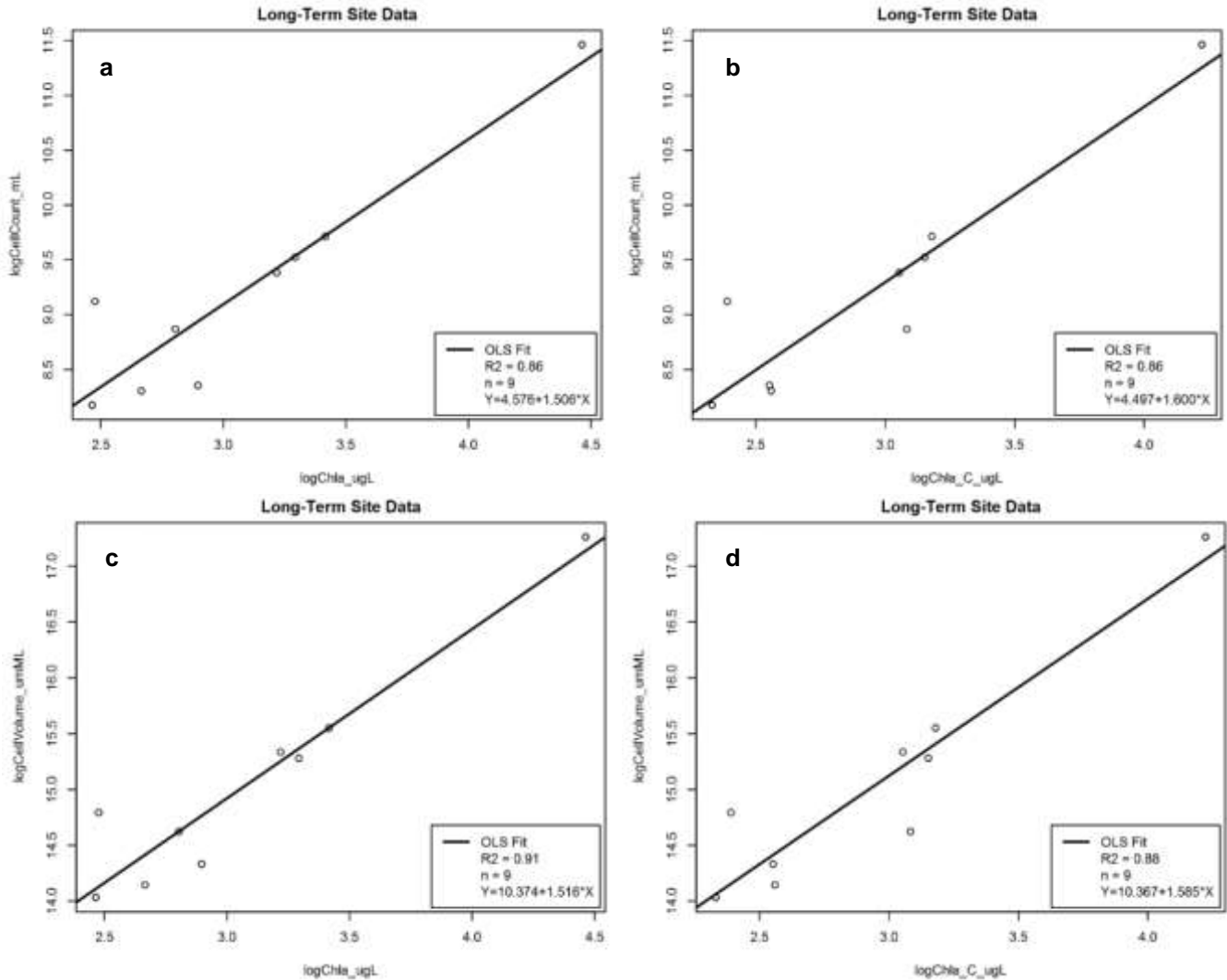
Figure 2.2.3. Relationship between (a) chlorophyll concentration and phytoplankton cell count, (b) corrected chlorophyll concentration and phytoplankton cell count, (c) chlorophyll concentration and phytoplankton cell volume, and (d) corrected chlorophyll concentration and phytoplankton cell volume. Points represent measurements made at sites averaged across all sampled dates.
