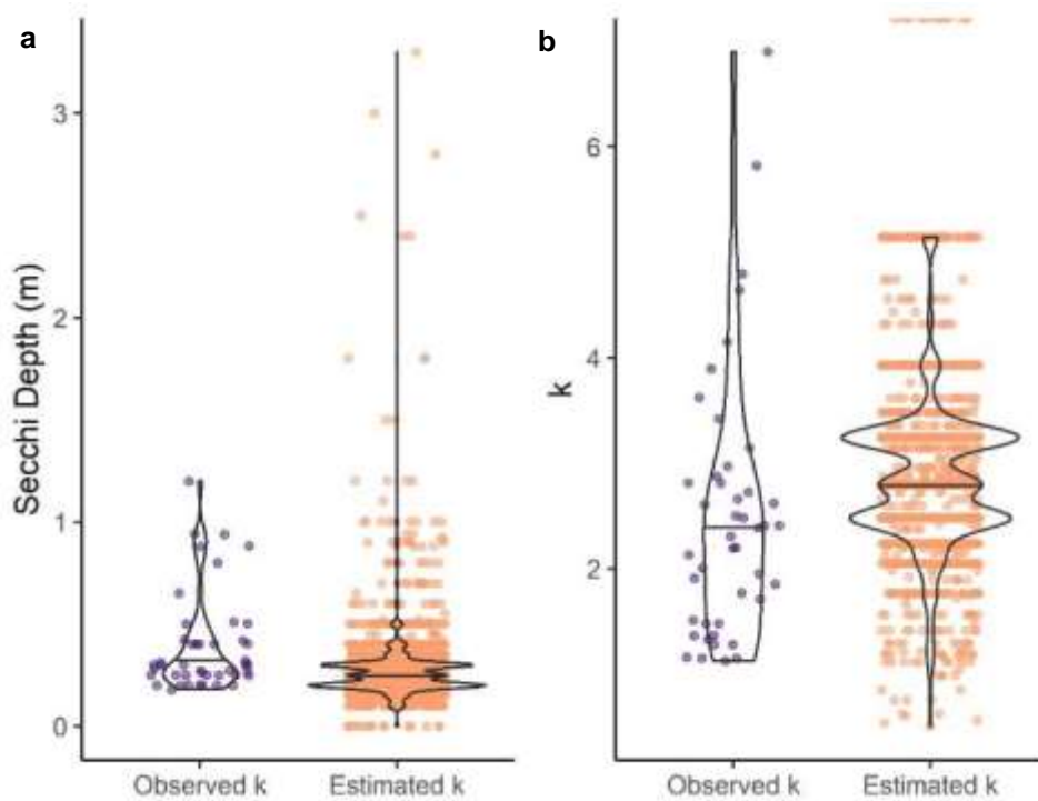
Figure 2.8.3. Relationship between Secchi depth and light attenuation coefficient ( k ) in Utah Lake.
