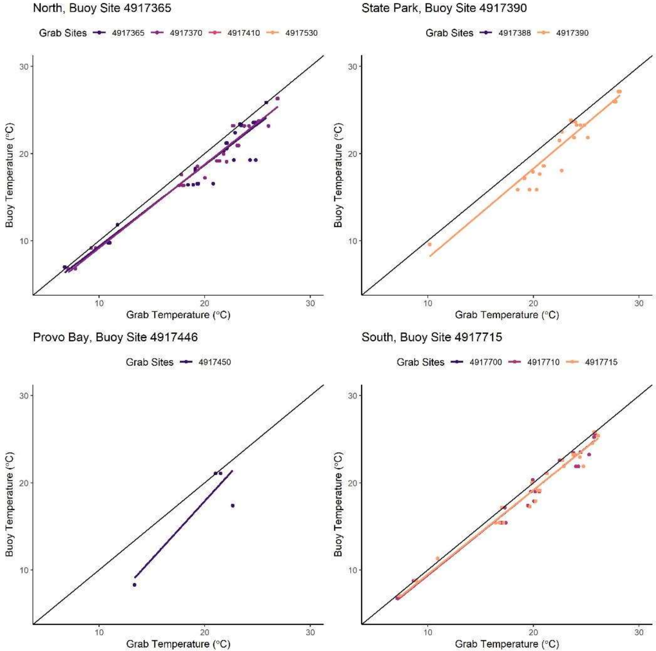
Figure 2.3.5. Comparisons of temperature measured at buoy and grab sampling sites. Grab sites correspond to sites near the buoy site, which did not necessarily have data available. A direct match in site code indicates grab and buoy samples were taken at the same location. The solid black line represents a 1:1 relationship.
