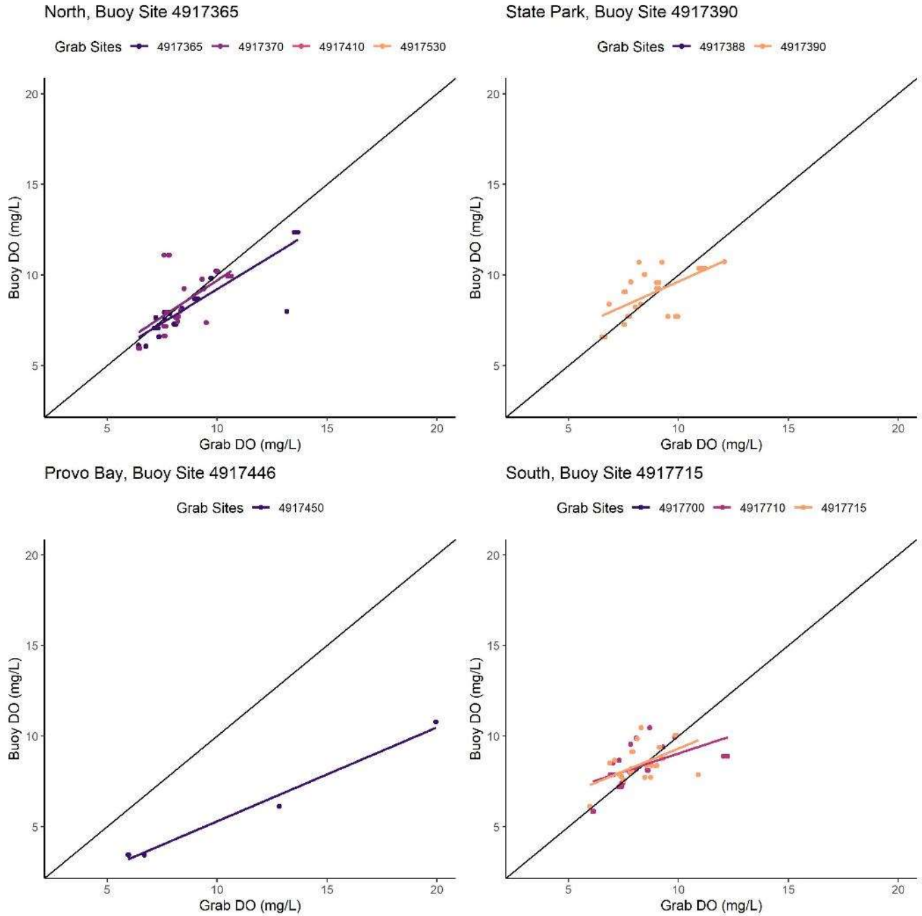
Figure 2.3.7. Comparisons of dissolved oxygen (DO) measured at buoy and grab sampling sites. Grab sites correspond to sites near the buoy site, which did not necessarily have data available. A direct match in site code indicates grab and buoy samples were taken at the same location. The solid black line represents a 1:1 relationship.
