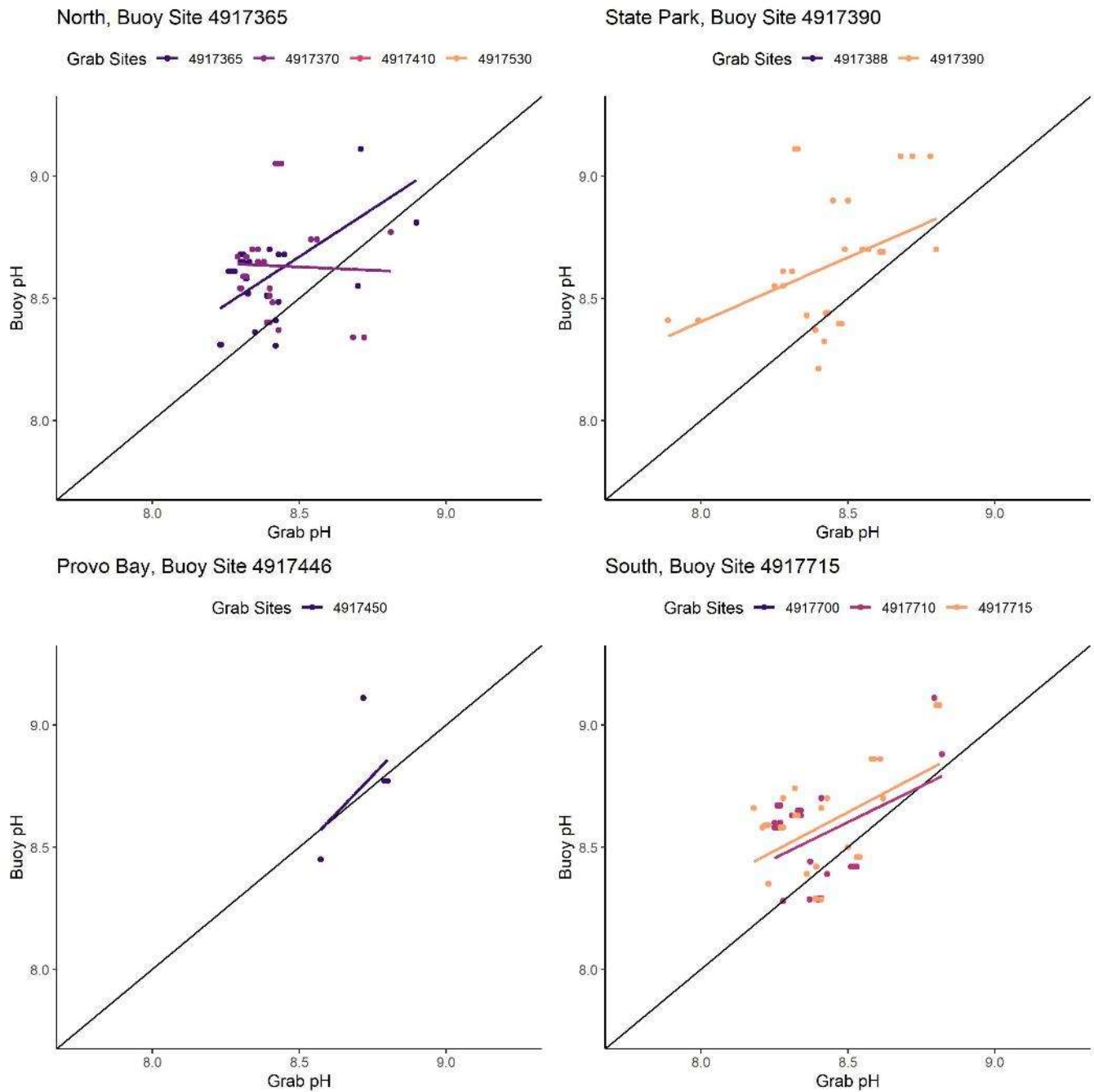
Figure 2.3.8. Comparisons of pH measured at buoy and grab sampling sites. Grab sites correspond to sites near the buoy site, which did not necessarily have data available. A direct match in site code indicates grab and buoy samples were taken at the same location. The solid black line represents a 1:1 relationship.
