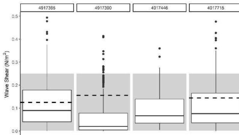
Figure 2.6.7. Observed wave shear in Utah Lake (boxplots) as compared to calculated critical shear values (dotted lines) and literature critical shear values from other systems (Chao et al. 2008). Site codes are as follows: North = 4917365, State Park = 4917390, Provo Bay = 4917446, South = 4917715.
