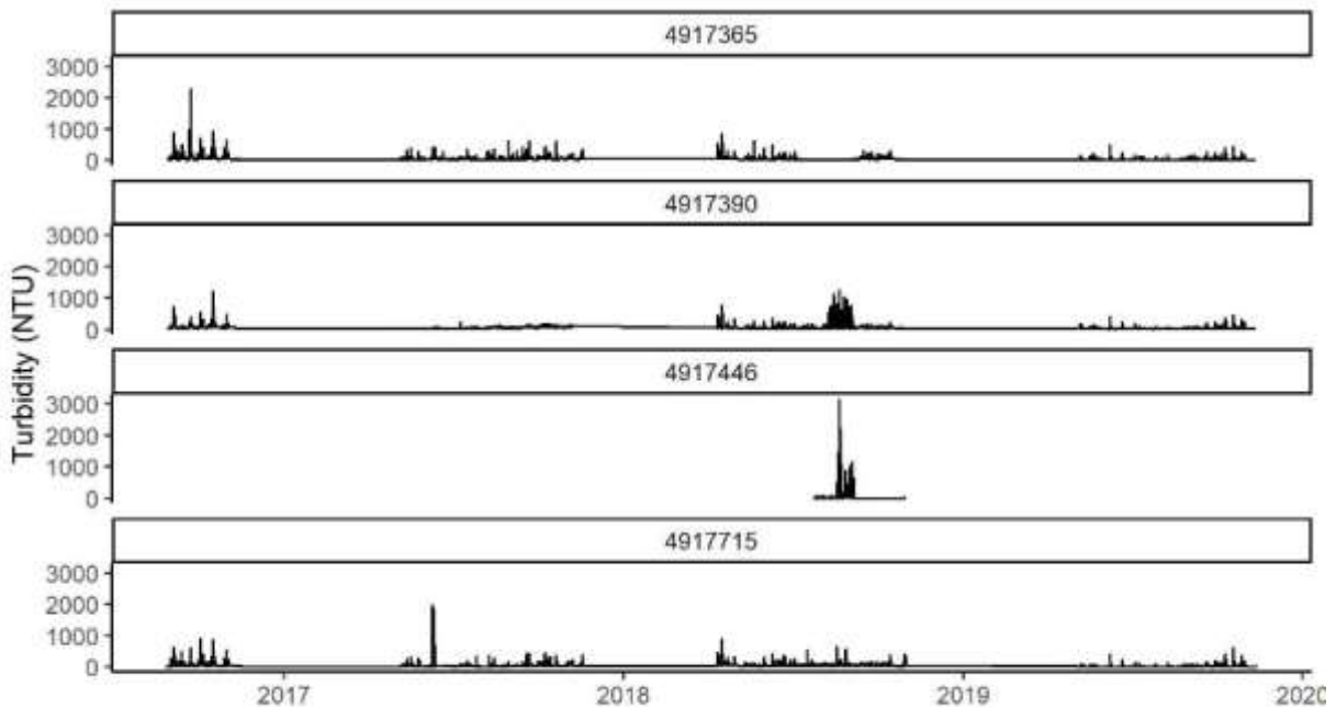
Figure 2.6.3. Time series of turbidity at buoy sites. Site codes are as follows: North = 4917365, State Park = 4917390, Provo Bay = 4917446, South = 4917715. NTU = nephelometric turbidity units. Horizontal lines at 0 NTU indicate a gap in sampling data, not an absence of turbidity.
