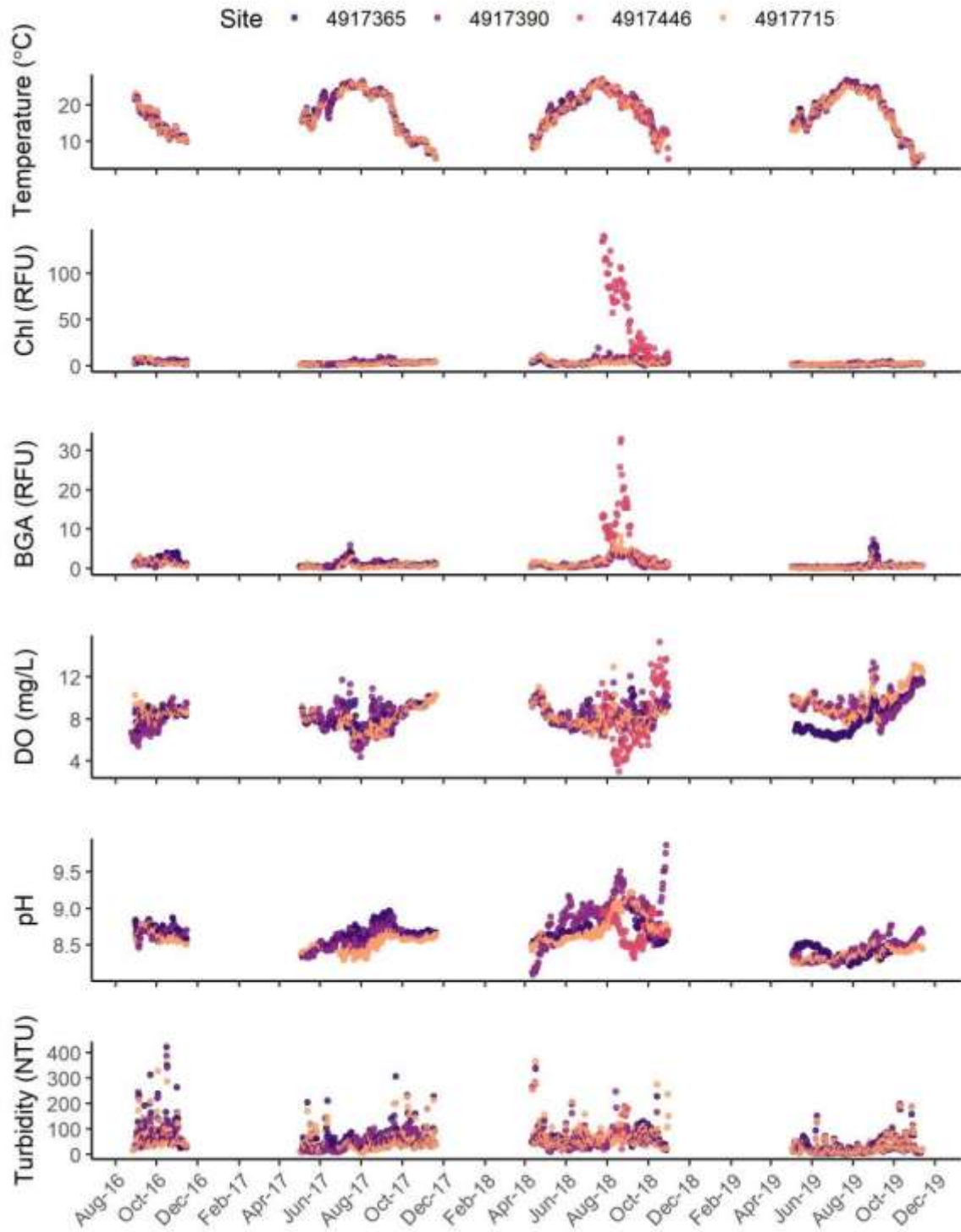
Figure 2.3.2. Time series of measured variables at buoy sites. Site codes are as follows: North = 4917365, State Park = 4917390, Provo Bay = 4917446, South = 4917715. Chl = chlorophyll, RFU = relative fluorescence units, BGA = blue-green algae, DO = dissolved oxygen, NTU = nephelometric turbidity units.
