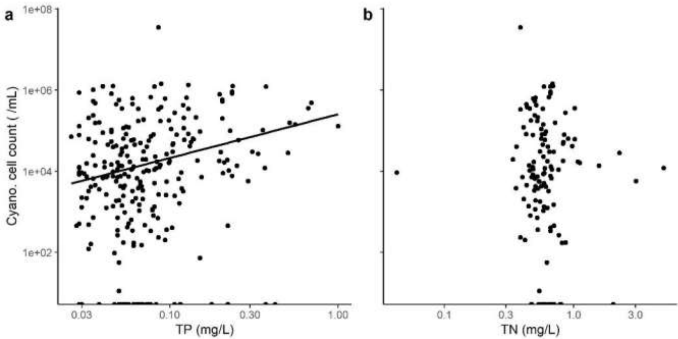
Figure 2.4.12. Relationships of cyanobacterial cell count to (a) TP and (b) TN. The line of best fit in (a) indicates a significant correlation. Note the logged axes for all variables.
