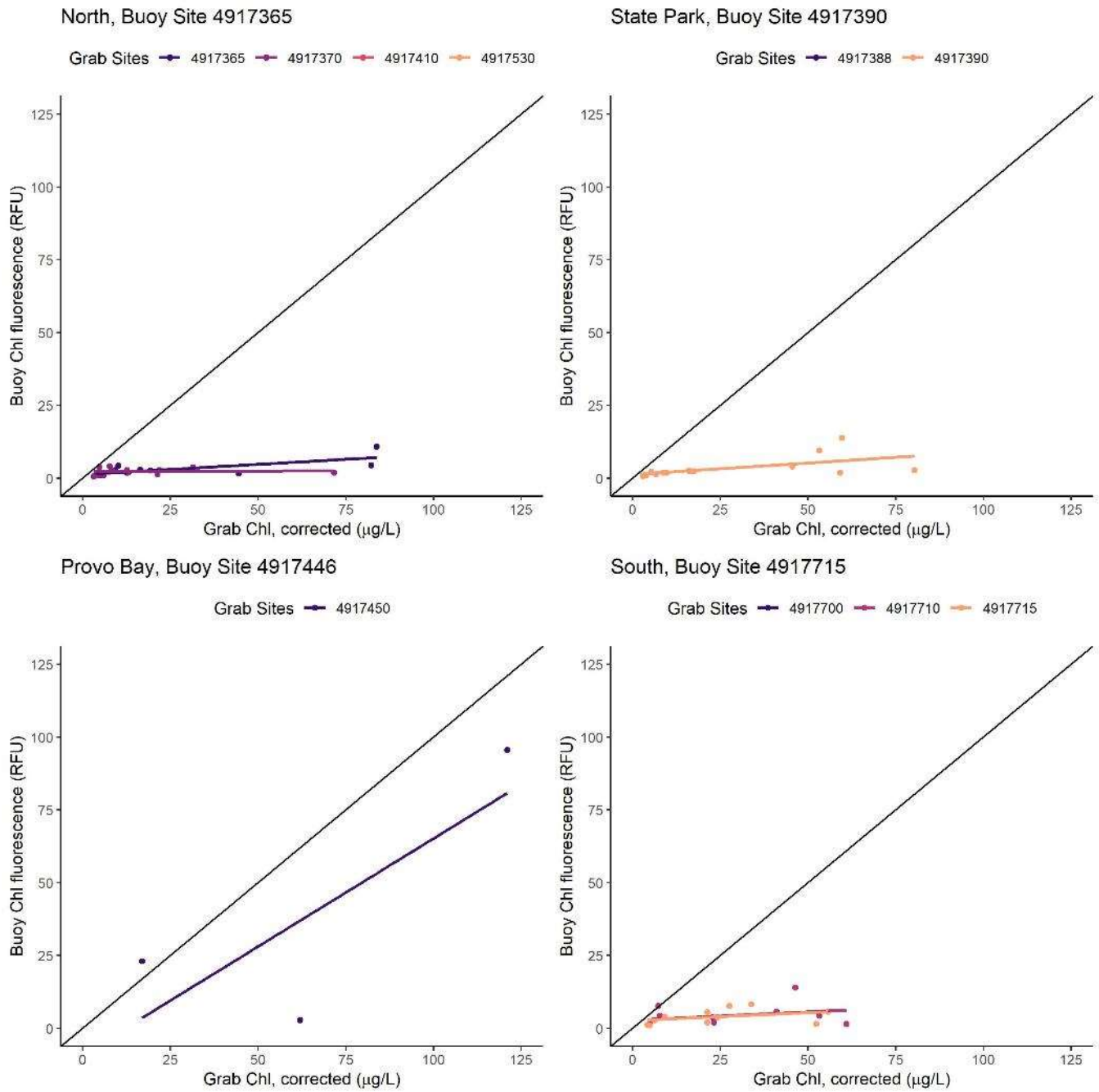
Figure 2.3.9. Comparisons of chlorophyll (chl) measured at buoy and grab sampling sites. Grab sites correspond to sites near the buoy site, which did not necessarily have data available. A direct match in site code indicates grab and buoy samples were taken at the same location. The solid black line represents a 1:1 relationship. RFU = relative fluorescence units.
