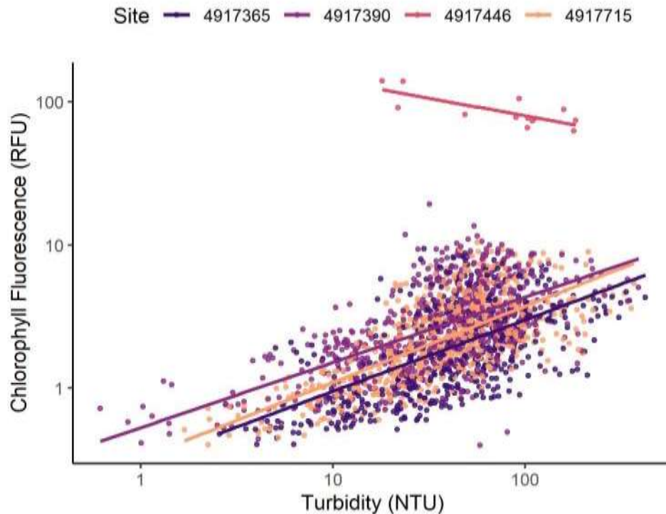
Figure 2.3.4. Correlation of turbidity and chlorophyll fluorescence at buoy sites. Site codes are as follows: North = 4917365, State Park = 4917390, Provo Bay = 4917446, South = 4917715. RFU = relative fluorescence units, NTU = nephelometric turbidity units.
