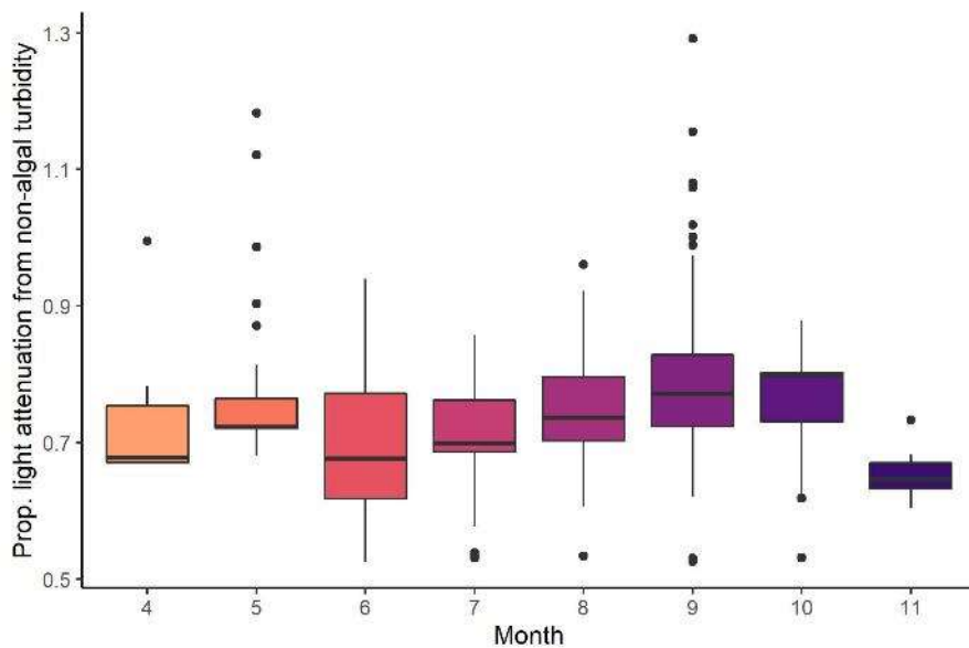
Figure 2.8.6. Proportion of total light attenuation contributed from non-algal turbidity.
